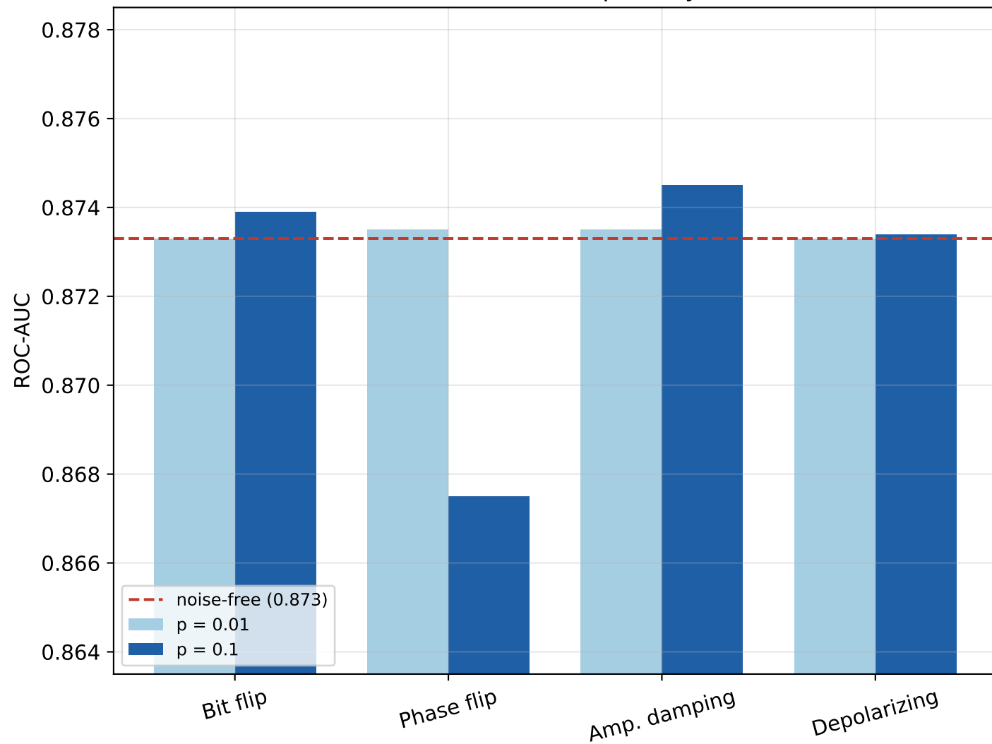
Azamuke 2024 (primary)
